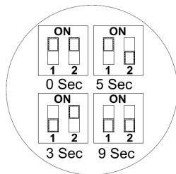
Auto Re-Locking Timer Settings
