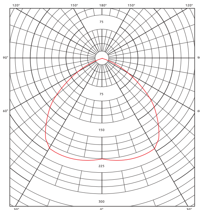
Light distribution curve per 1000 lumens
