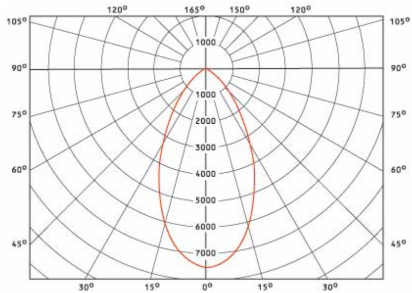
light distribution curve (high bay lighting)
