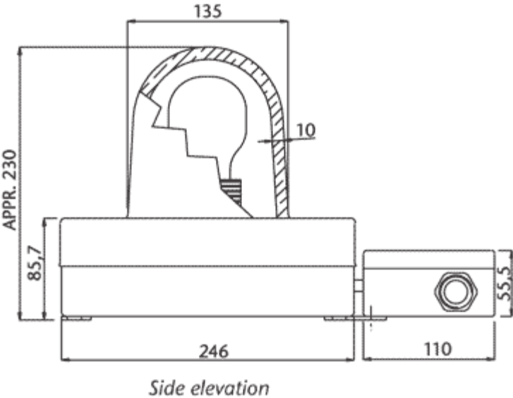
IQL55 detail light drawing
