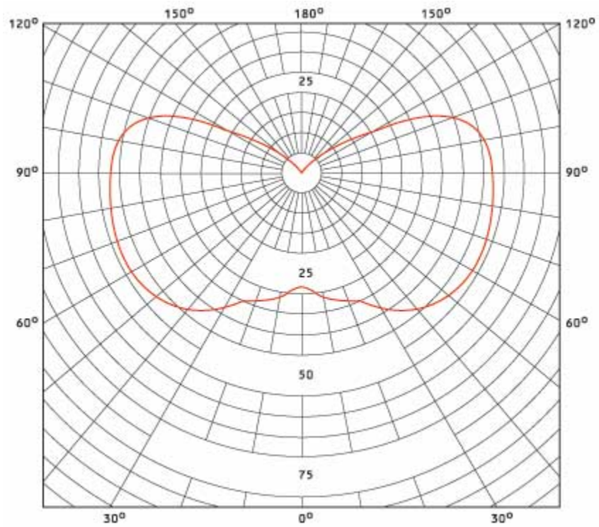
Light distribution curve
