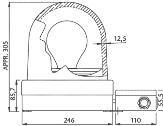
Side elevation
