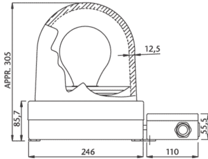
Side elevation
