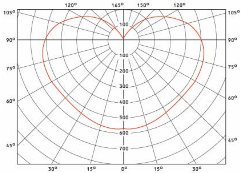
Light Distribution curve (Frosted)
