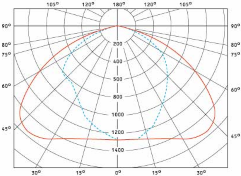
Light Distribution curve (area lighting)
