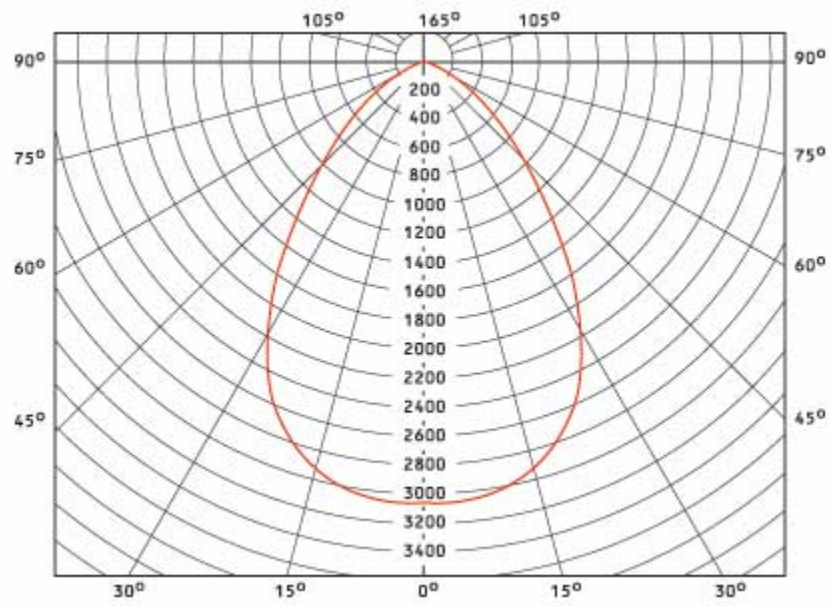
light distribution curve (high bay lighting)
