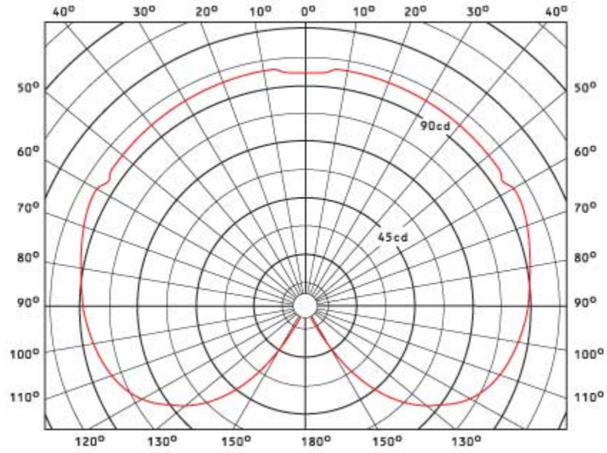
light distribution curve (Obstruction)
