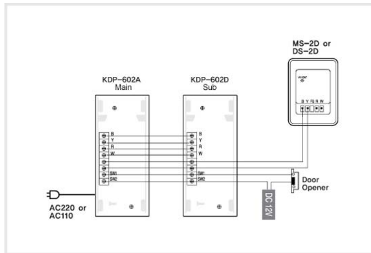
KDP-602AD wiring diagram
