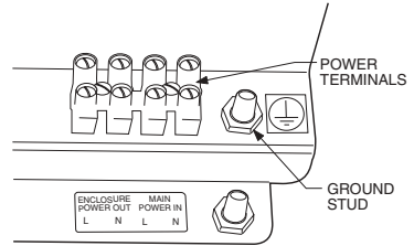
Figure 3. ERD2200 Power Connections
